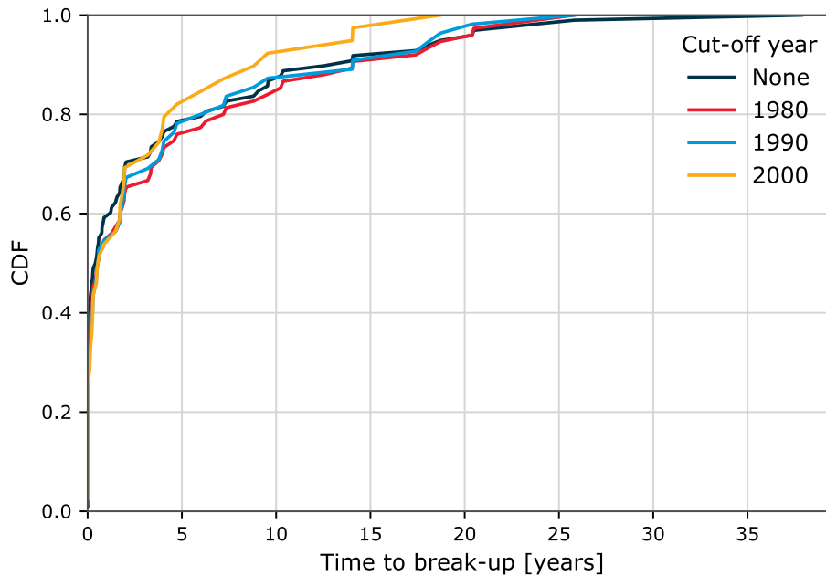
Figure 5.8: Cumulative distribution function for the elapsed time between fragmentation and launch for non-system related fragmentation events, with different cut-off values on the launch year.
