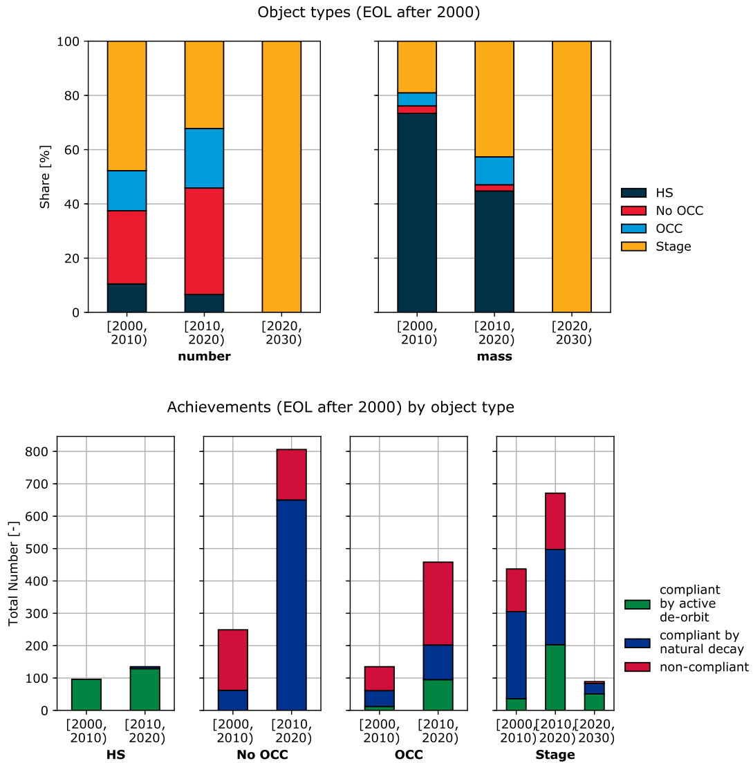
Figure 6.1: Share of payload and rocket bodies in terms of mass and number (top) and compliance in terms of clearing the LEO protected region (bottom). The reported years for payload clearance of LEO IADC goes up to 2019, for rocket body clearance of LEO IADC goes up to 2020.
