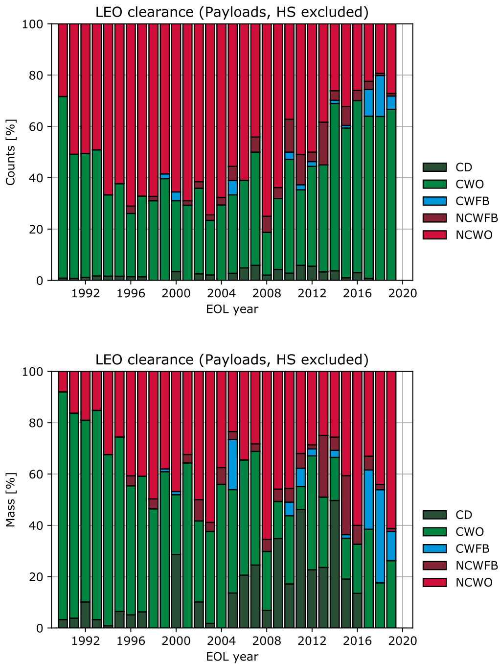
Figure 6.4: Relative share of disposal behaviour classes over time in terms of number (top) and mass (bottom) for payloads in LEO, excluding objects associated with human spaceflight.
