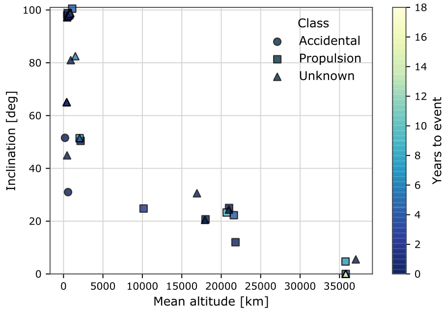
Figure 5.9: Distribution of non-system related fragmentation events in mean altitude, inclination, and time to fragmentation.
