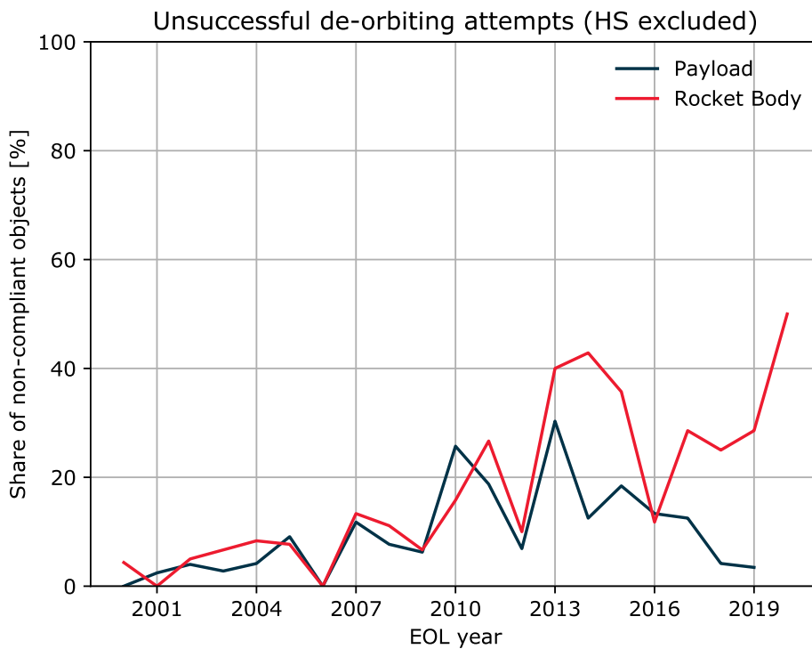
Figure 6.7: Relative shares of success w.r.t. compliance (top) and non-compliance (bottom) over time, excluding objects associated with human spaceflight.
