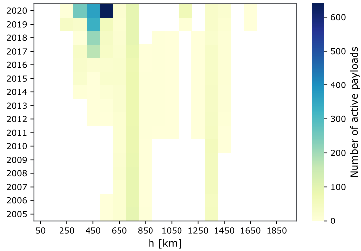
Figure 2.19: Distribution of active payloads belonging to constellations in LEO by year and mean altitude.
