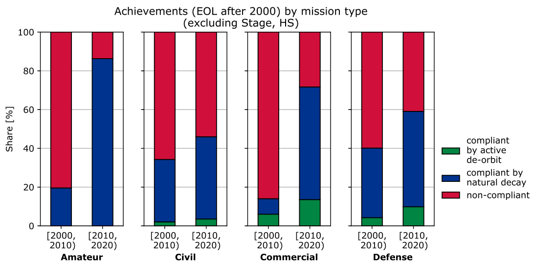
Figure 6.2: Share of compliance in terms of clearing the LEO protected region by mission type.
