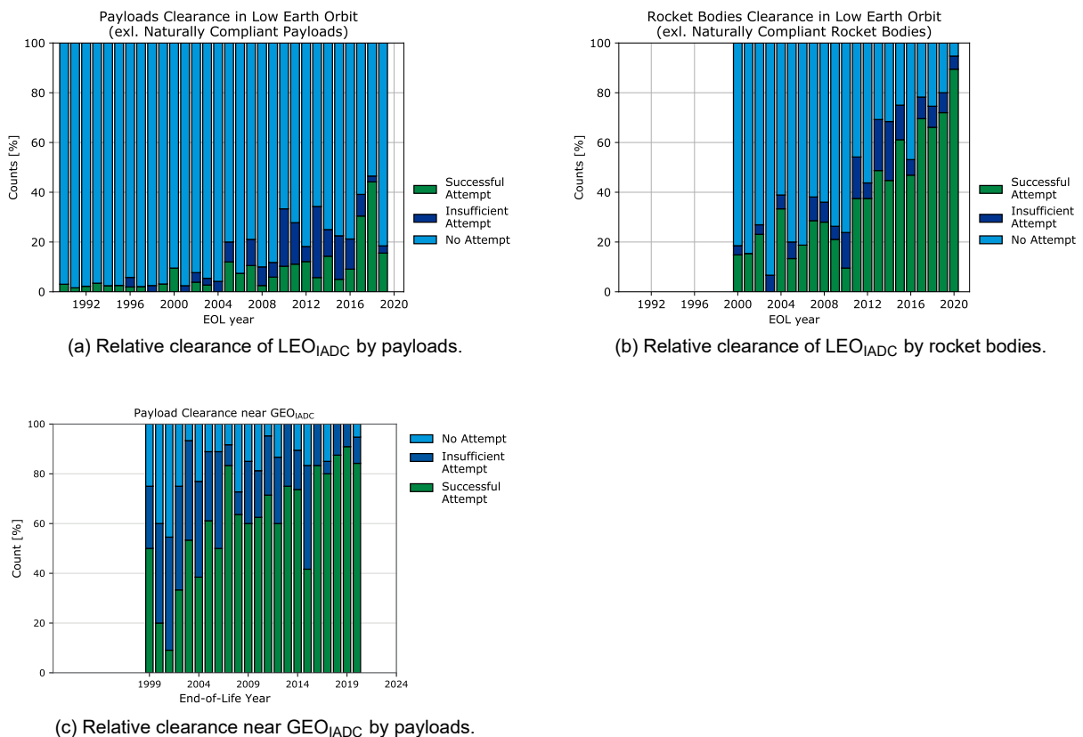
Figure 5: Trend of adherence to clearance of the protected region over time in terms of numbers, excluding naturally compliant objects.
