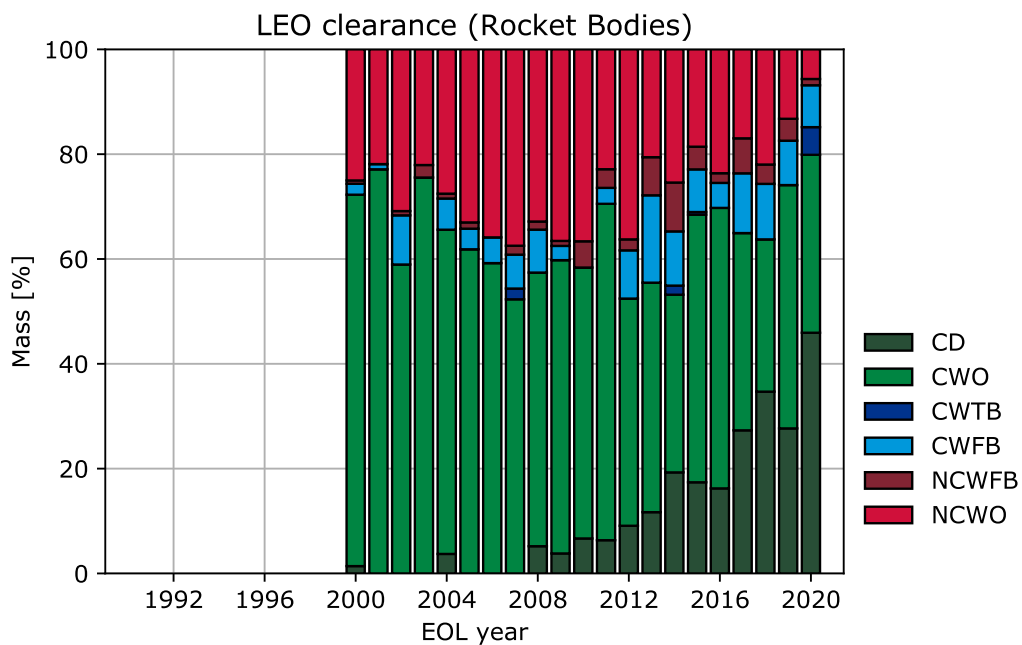
Figure 6.6: Relative share of disposal behaviour classes over time in terms of number (top) and mass (bottom) for Rocket Bodies in LEO.
