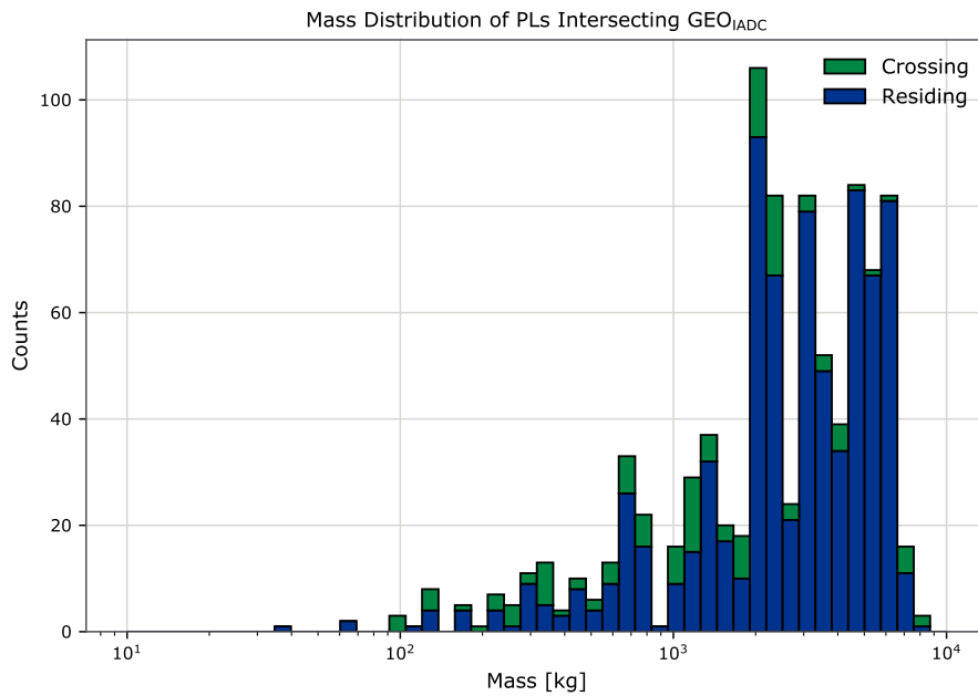
(a) Mass histogram of payloads in GEO.
