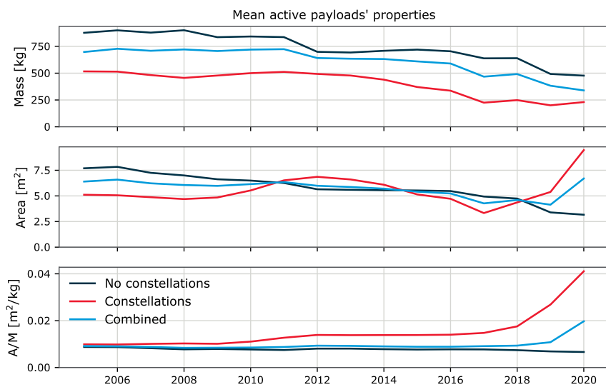
Figure 2.20: Payload parameters for active payloads in LEO over time.
