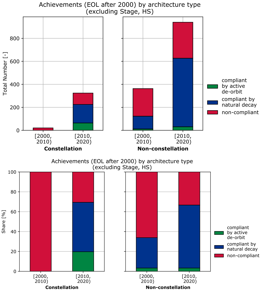
Figure 6.3: Compliance in terms of clearing the LEO protected region for constellation and non-constellation objects, in absolute numbers and in relative share.
