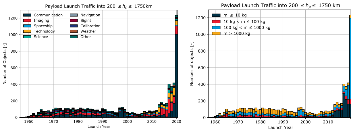
Figure 2: Evolution of the launch traffic near LEO IADC per mission type (left) and mass category (right).
