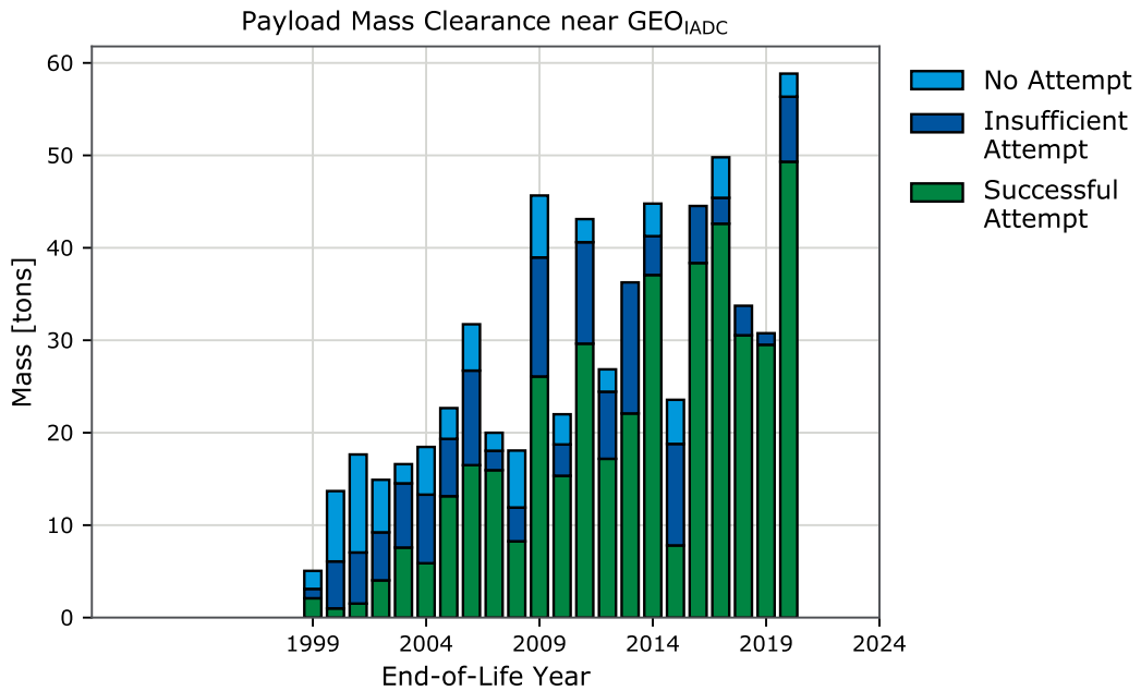
(a) Absolute mass clearance near GEO IADC .
