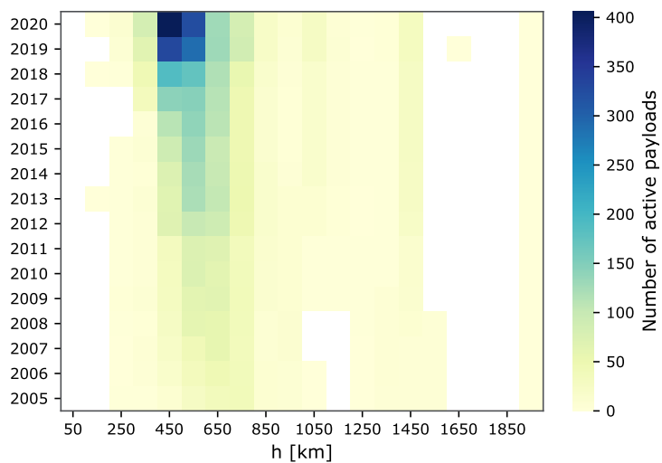
Figure 2.18: Distribution of active payloads not belonging to constellations in LEO by year and mean altitude.
