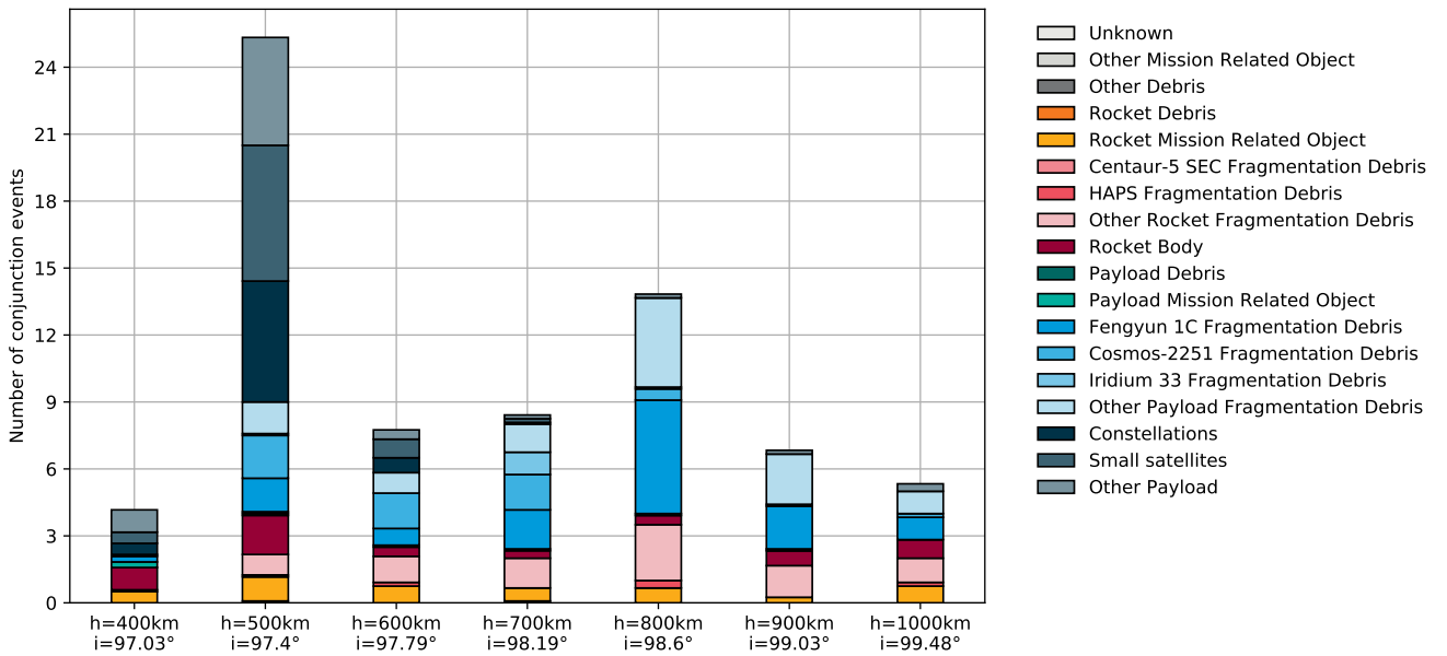
Figure 3.11: Conjunction events, and chaser classification, for a set of representative missions in Sun-synchronous orbits over 2020.
