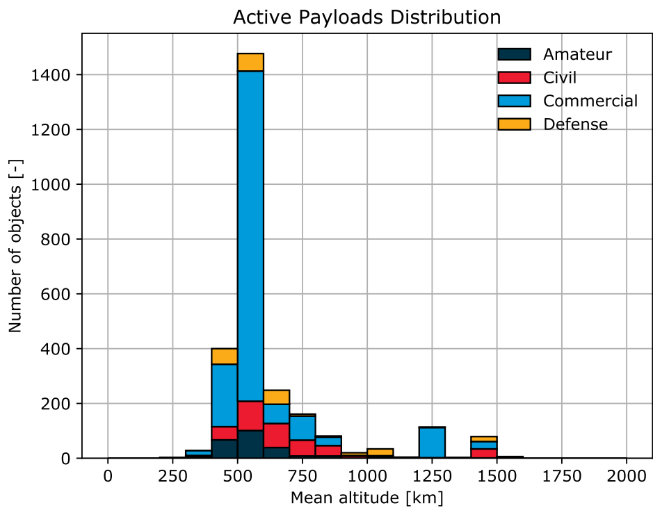
Figure 3.6: Launch traffic in 2020 (top) and distribution of active payloads (bottom) in LEO IADC by mean altitude.
