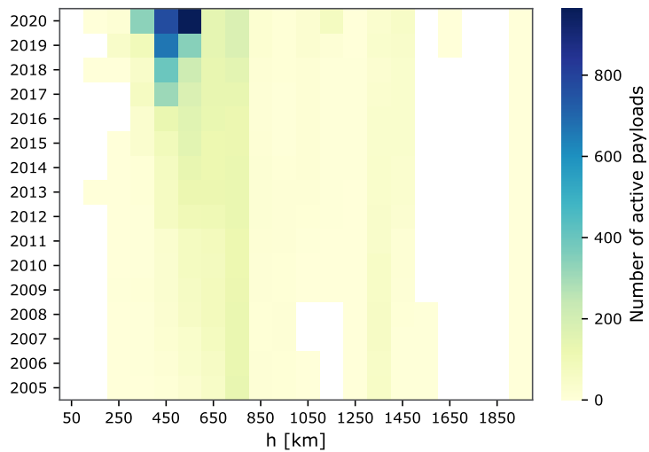
Figure 2.17: Distribution of active payloads in LEO by year and mean altitude.
