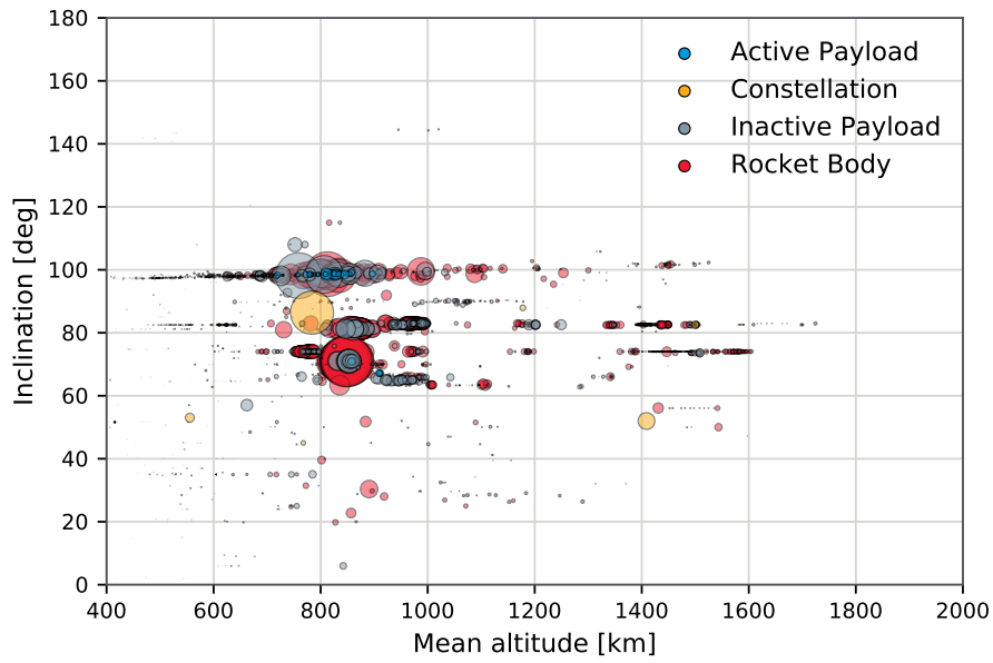
Figure 7.1: Index value for objects in LEO. The size of the marker is proportional to the debris index of the object or constellation.
