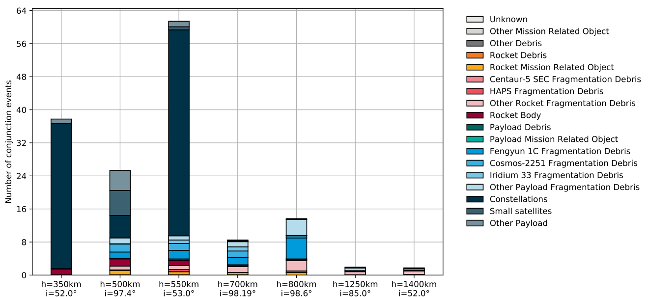
Figure 3.10: Conjunction events, and corresponding chaser classification, for a set of representative missions over 2020.
