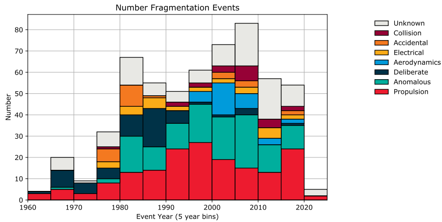
Figure 3: Historical trend of fragmentation events per event cause. The last bin covers only the year 2020.
