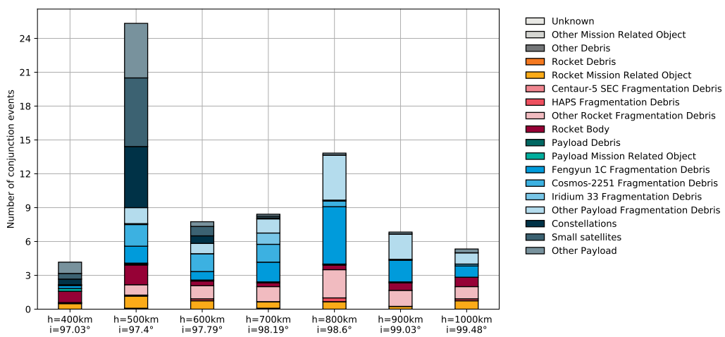
Figure 6: Close approaches, and chaser classification, for a set of representative missions in Sun-synchronous orbits over 2020.
