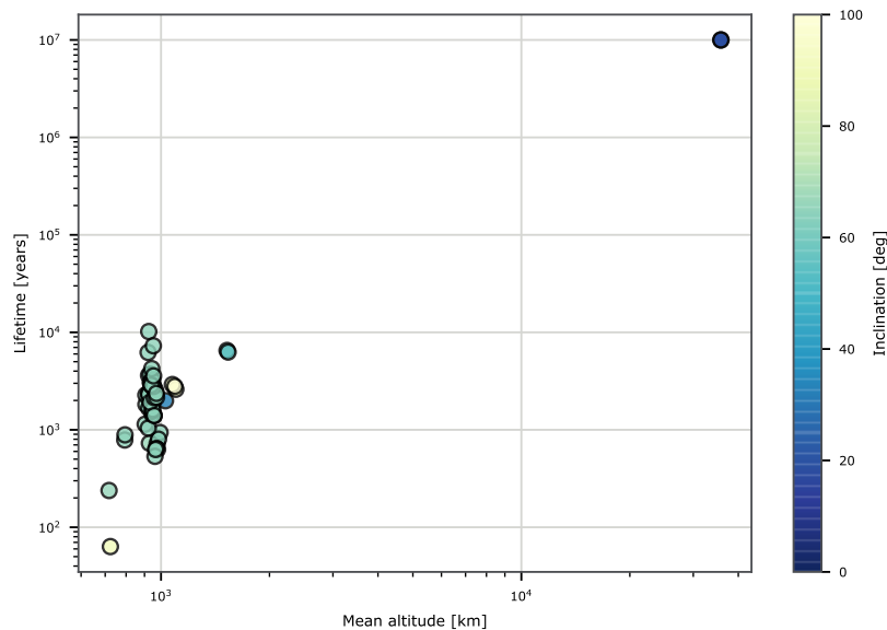
Figure 2.27: Distribution of space objects with nuclear power sources with mean altitude, orbital lifetime, and inclination.
