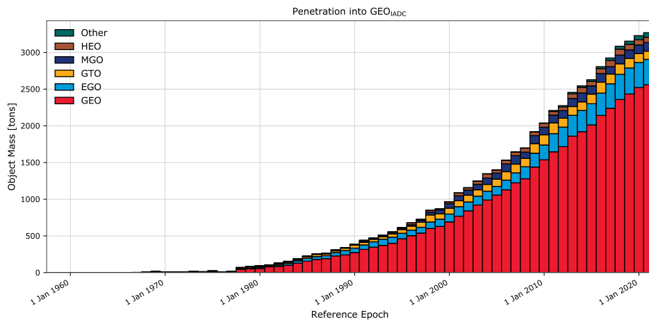
(b) Evolution of absolute mass.
