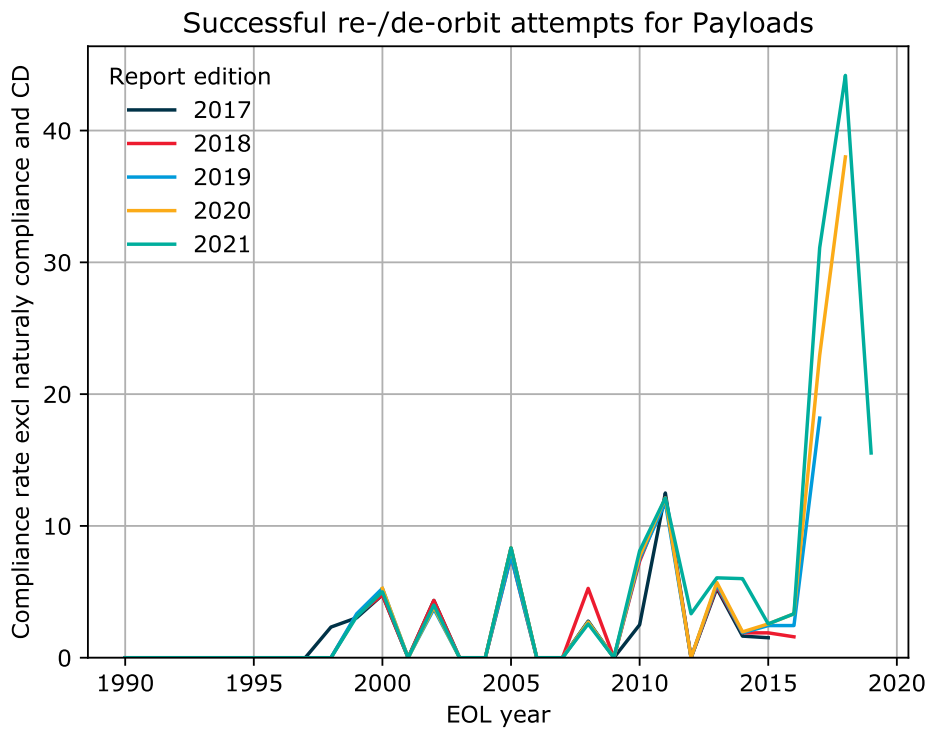
Figure 6.17: Successful re-/de-orbit attempts for payloads according to the different report editions.
