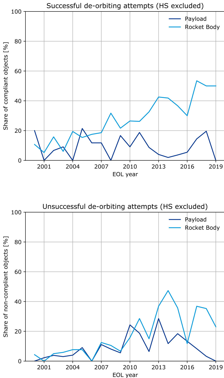
Figure 6.6: Relative shares of success w.r.t. compliance (top) and non-compliance (bottom), excluding objects associated with human spaceflight.
