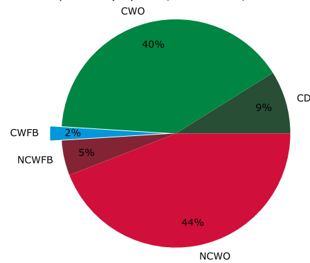
LEO compliances (Payloads, EOL \geq 2000, m > 1000 kg)
