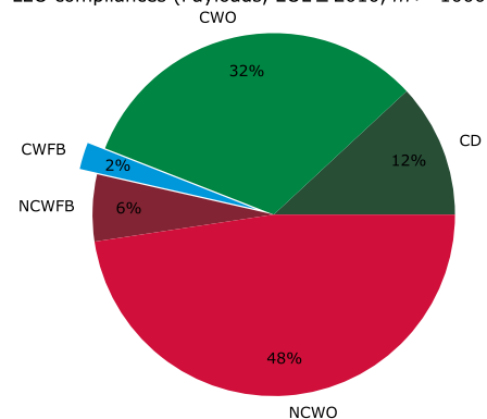
LEO compliances (Payloads, EOL \geq 2010, m > 1000 kg)
