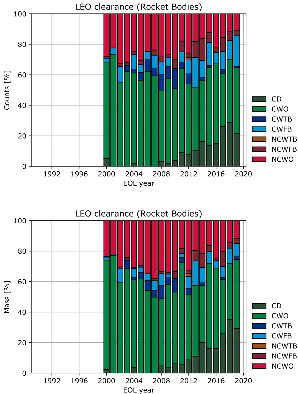
Figure 6.5: Relative share in terms of number (top) and mass (bottom) of disposal behaviour classes for Rocket Bodies in LEO.
