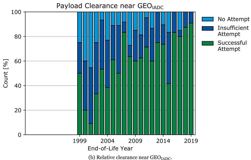
Figure 6.18: Trend of adherence to the disposal guideline in GEO_{IADC} .
