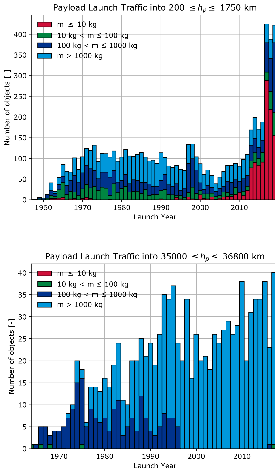
Figure 2.13: Evolution of the launch traffic per mass category in terms of number of objects in LEO IADC (top) and GEO IADC (bottom).
