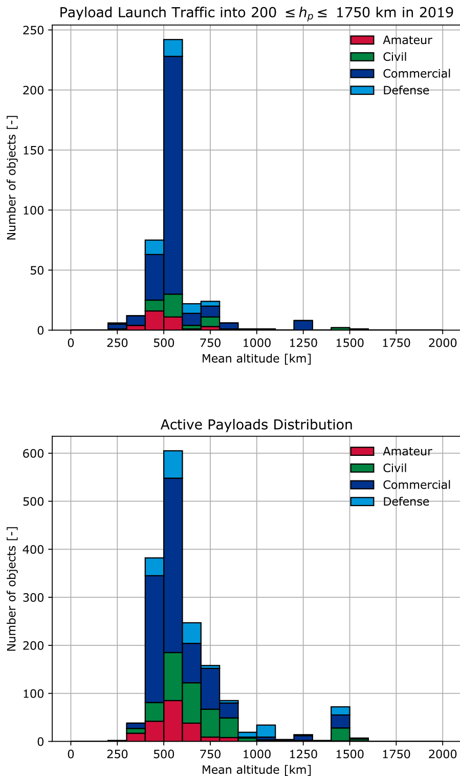
Figure 3.6: Launch traffic in 2019 (top) and distribution of active satellites (bottom) in LEO IADC by mean altitude.
