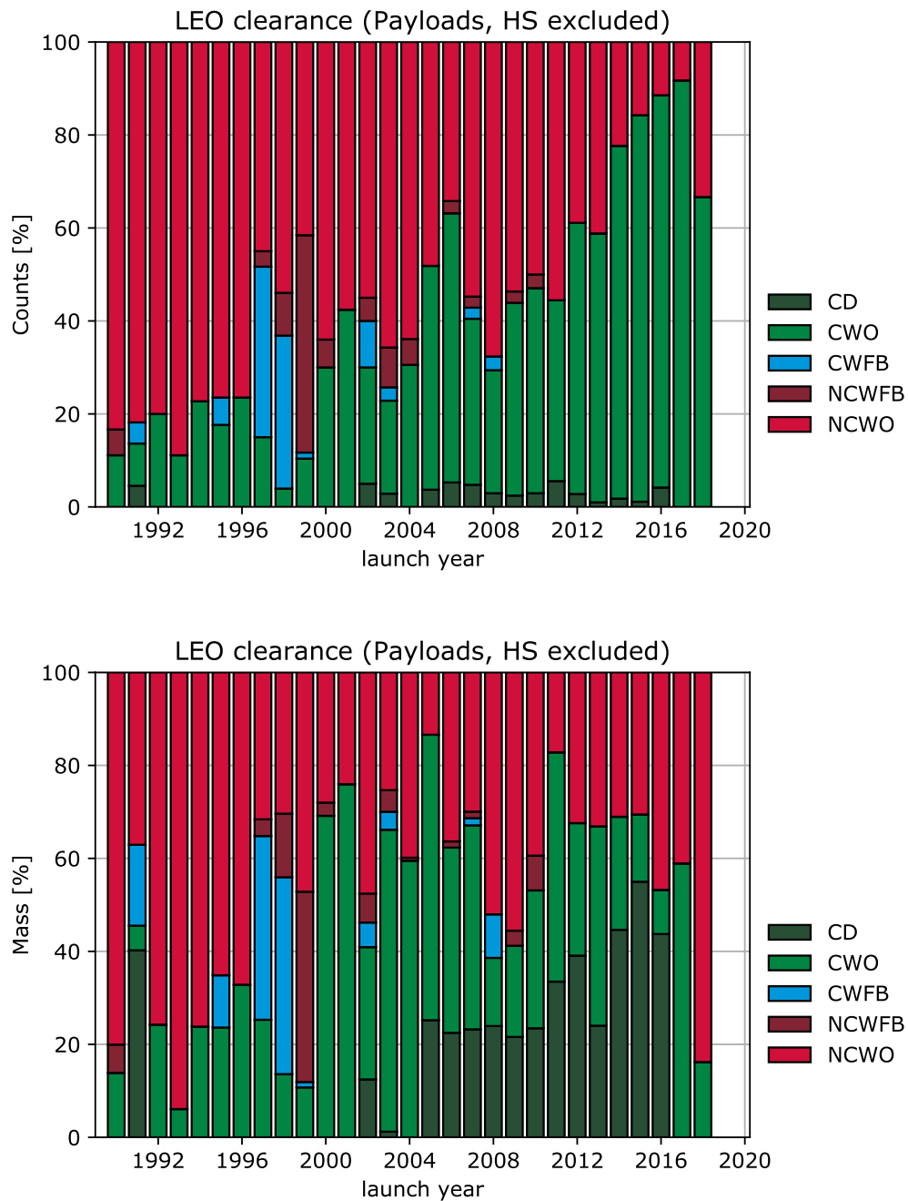
Figure 6.4: Relative share in terms of number (top) and mass (bottom) of disposal behaviour classes for payloads in LEO, excluding objects associated with human spaceflight by launch year.
