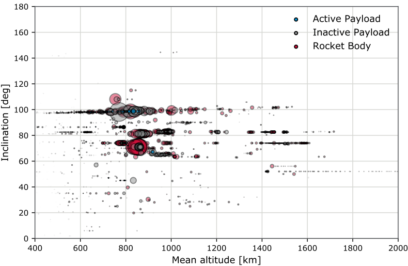
Figure 7.1: Index value for objects in LEO.
