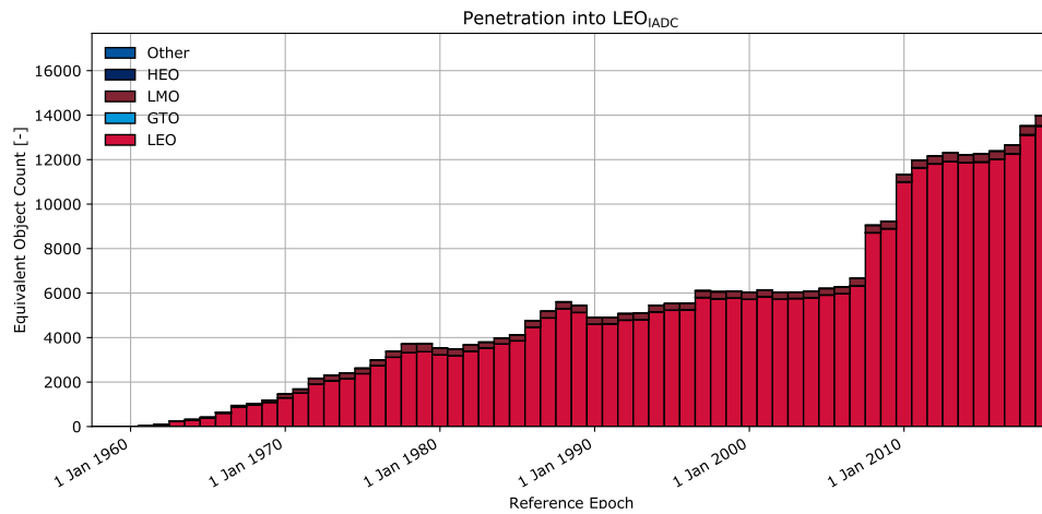
(a) Evolution of equivalent number of objects.
