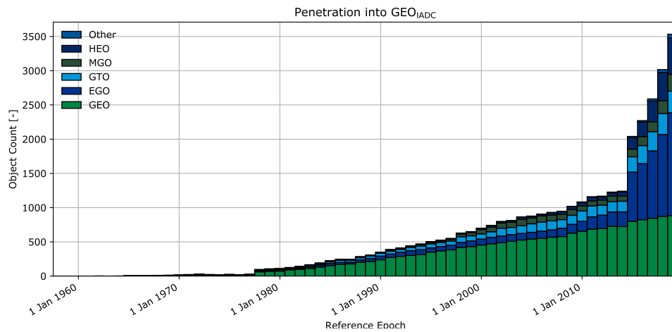
(a) Evolution of absolute number of objects.
