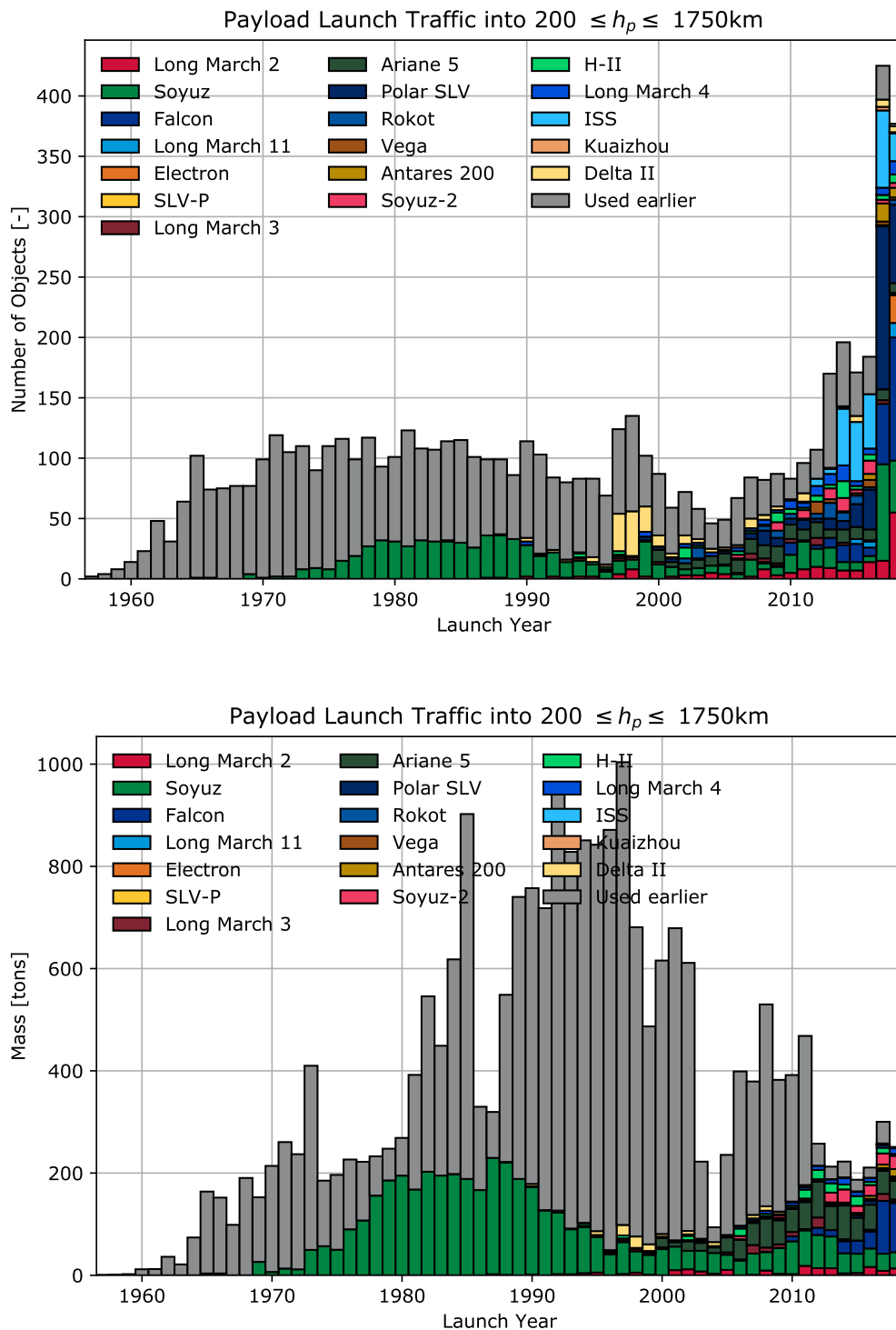
Figure 2.9: Evolution of the launch traffic near LEO_{IADC} per launcher family expressed in terms of number of objects (top) and mass (bottom).
