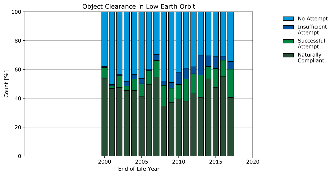
(a) Relative clearance of LEO IADC .
