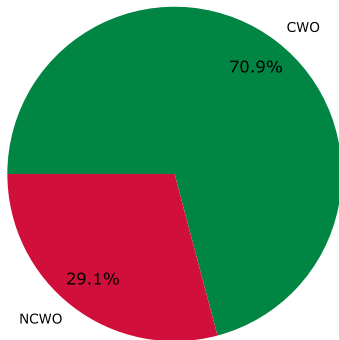
LEO compliances (Payloads w/o HS, EOL \geq 2000, m \leq 10kg)
