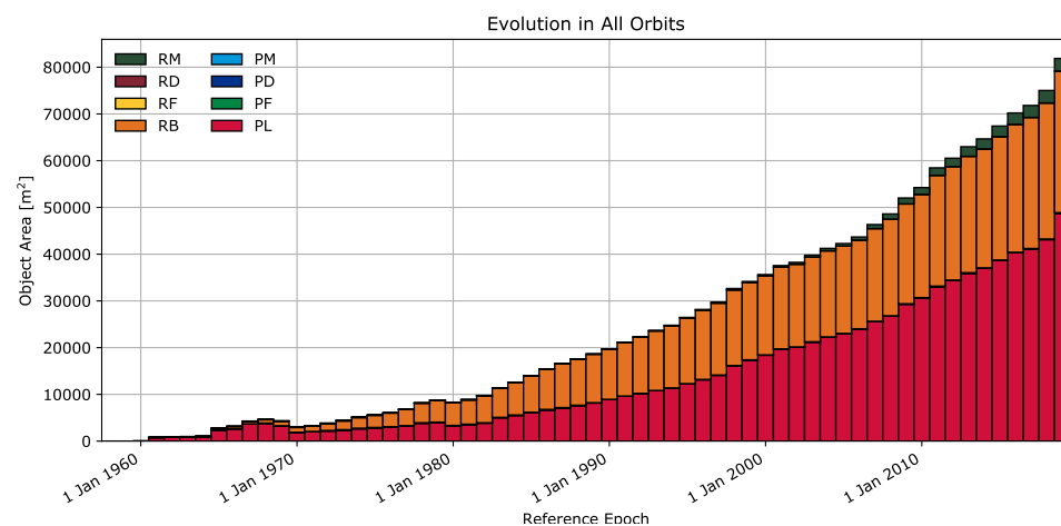
(c) Evolution of area.
