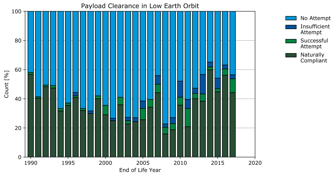
(a) Relative clearance of LEO IADC by payloads.
