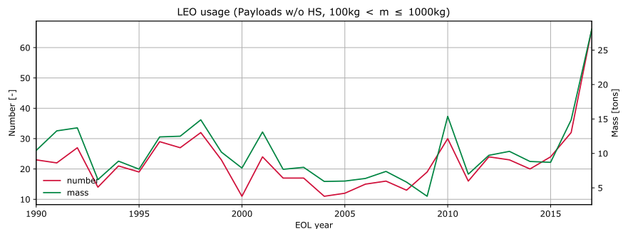
(c) Between 100.0 and 1000.0 kg
