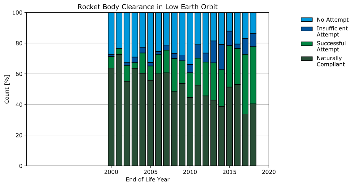
(b) Relative clearance of LEO IADC by rocket bodies.
