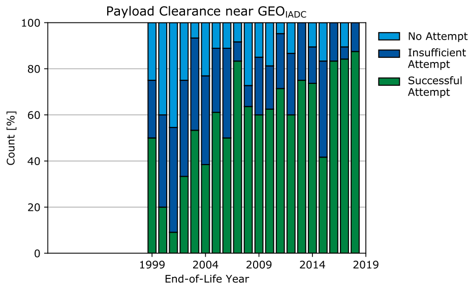
(b) Relative clearance near GEO IADC .
