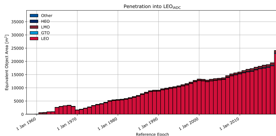
(c) Evolution of equivalent area.
