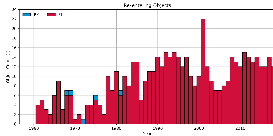
(a) Evolution of re-entered numbers.
