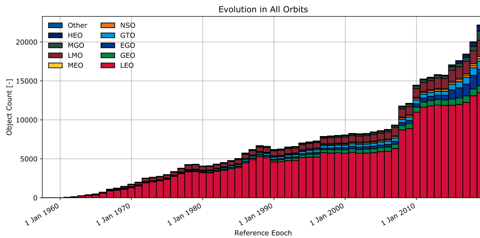
(a) Evolution of number of objects.
