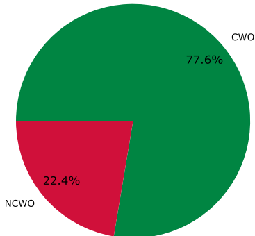
LEO compliances (Payloads w/o HS, EOL \geq 2010, m \leq 10kg)
