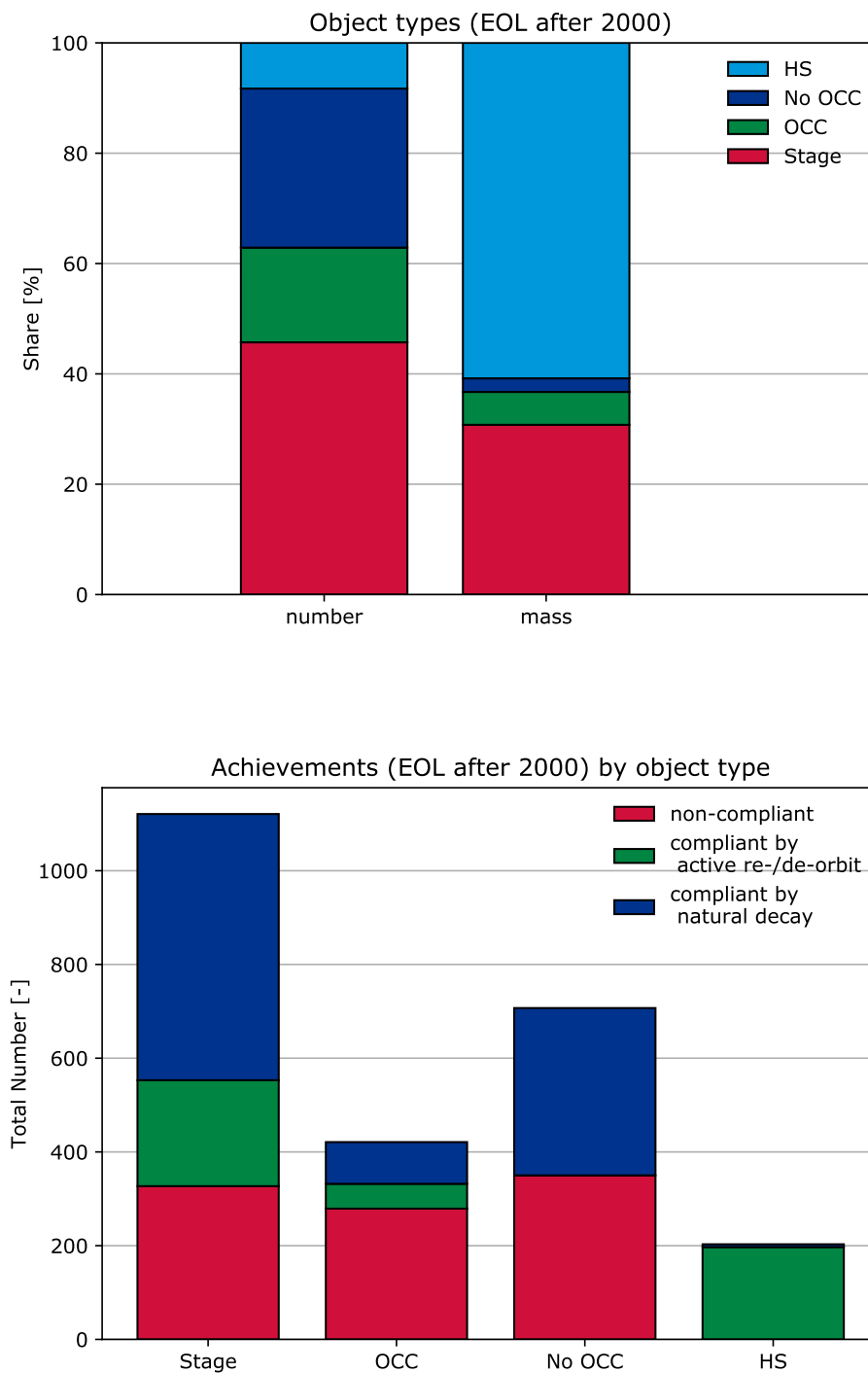
Figure 6.1: Share of payload and rocket bodies in terms of mass and number (top) and compliance in terms of clearing the LEO protected region (bottom).
