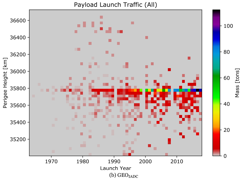
Figure 2.13: Evolution of the launch traffic: mass injected.
