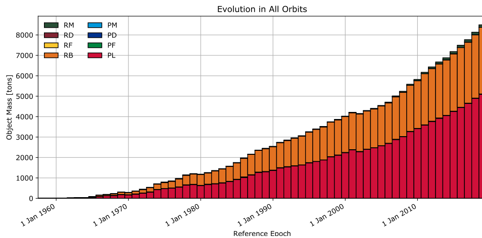
(b) Evolution of mass.
