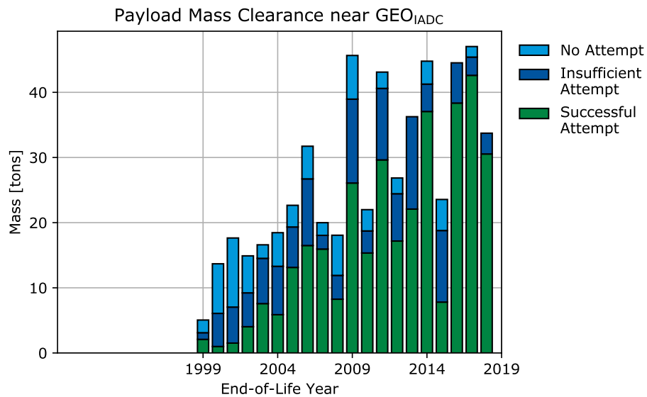
(a) Absolute mass clearance near GEO IADC .
