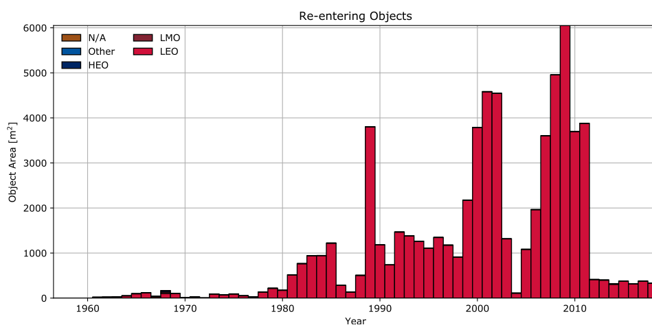
(c) Evolution of re-entered area.
