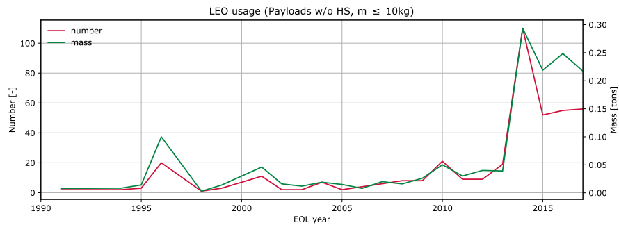
(a) Less than 10.0 kg.
