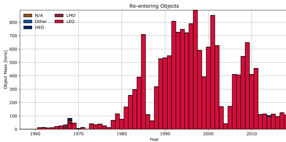
(b) Evolution of re-entered mass.
