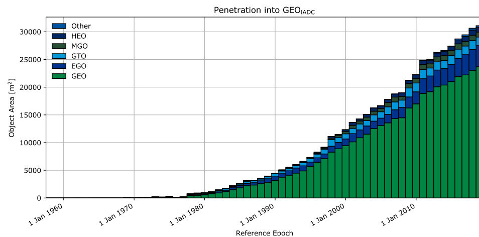
(c) Evolution of absolute area.
