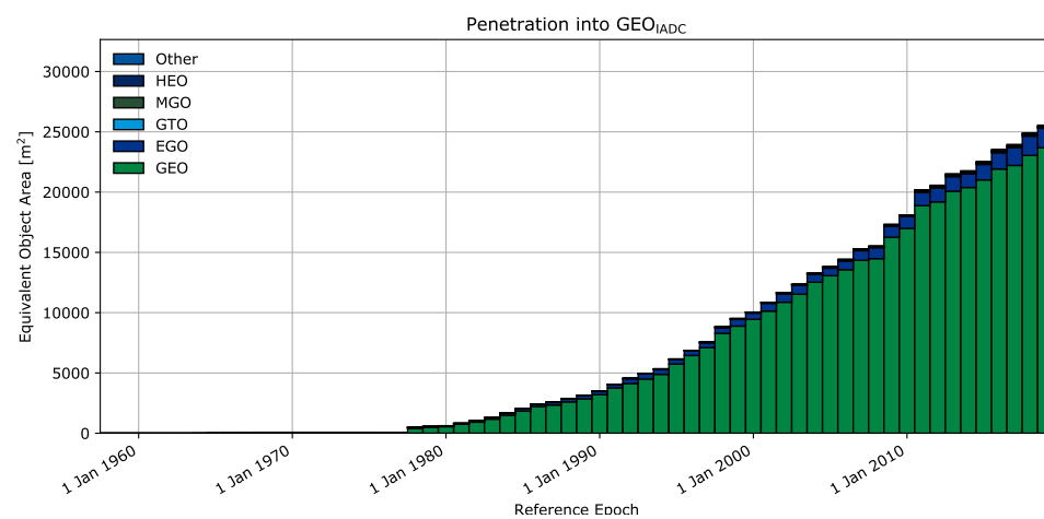
(c) Evolution of equivalent area.
