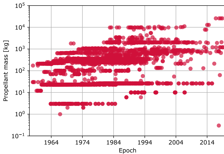
Figure 4.4: Evolution solid rocket motor firings.
