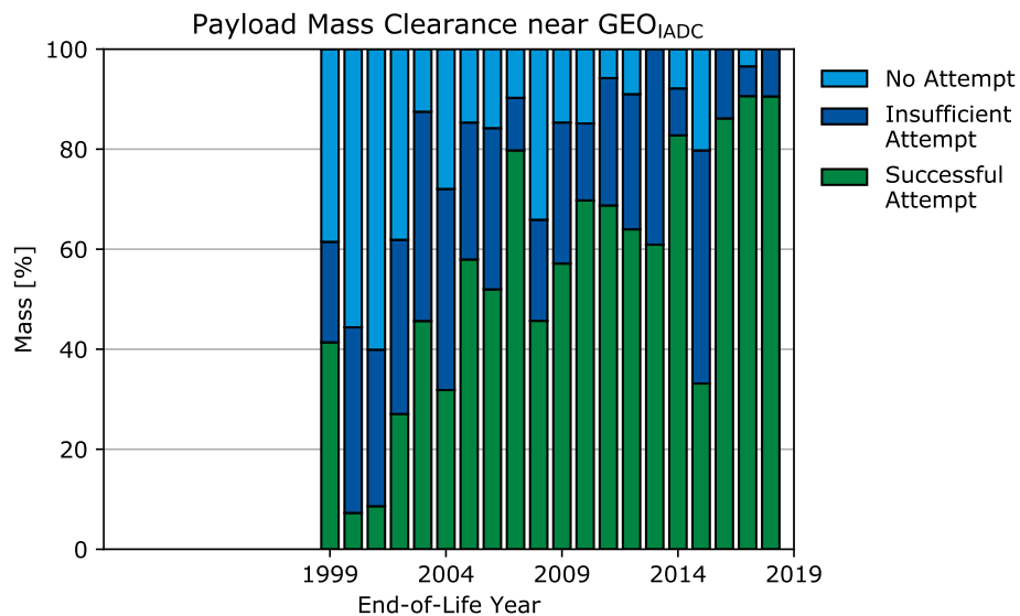
(b) Relative mass clearance near GEO IADC .
