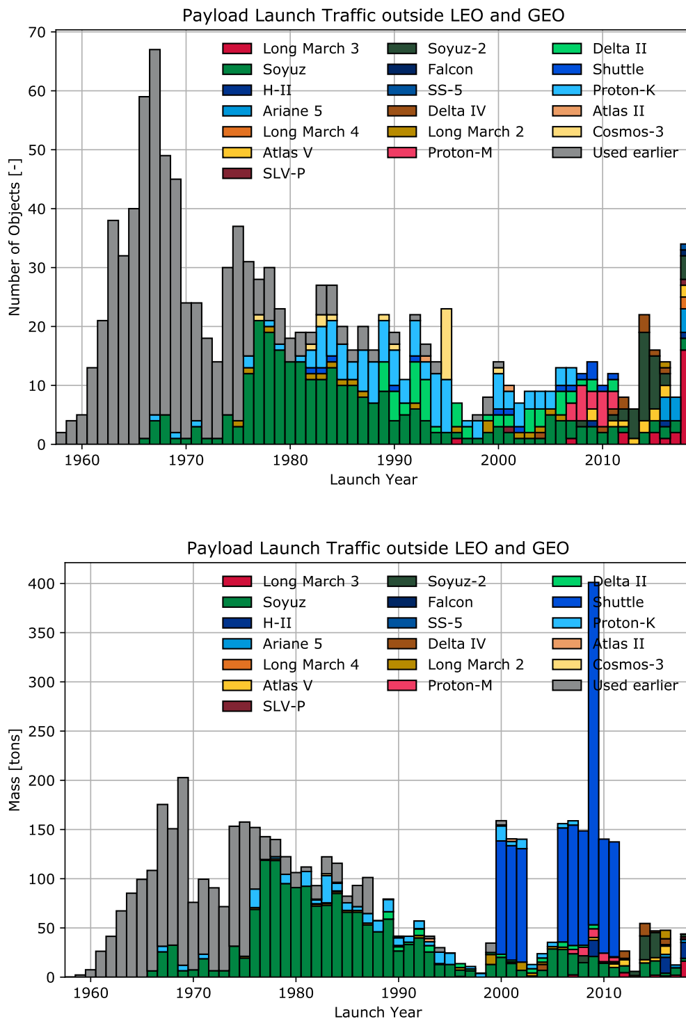
Figure 2.12: Evolution of the launch traffic outside LEO IADC and GEO IADC per launcher family expressed in terms of number of objects (top) and mass (bottom).
