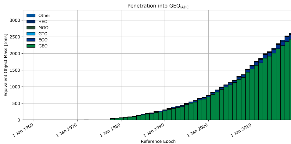
(b) Evolution of equivalent mass.
