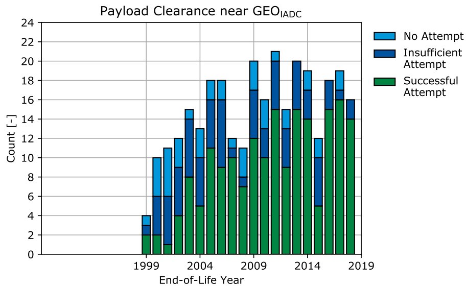
(a) Absolute clearance near GEO IADC .
