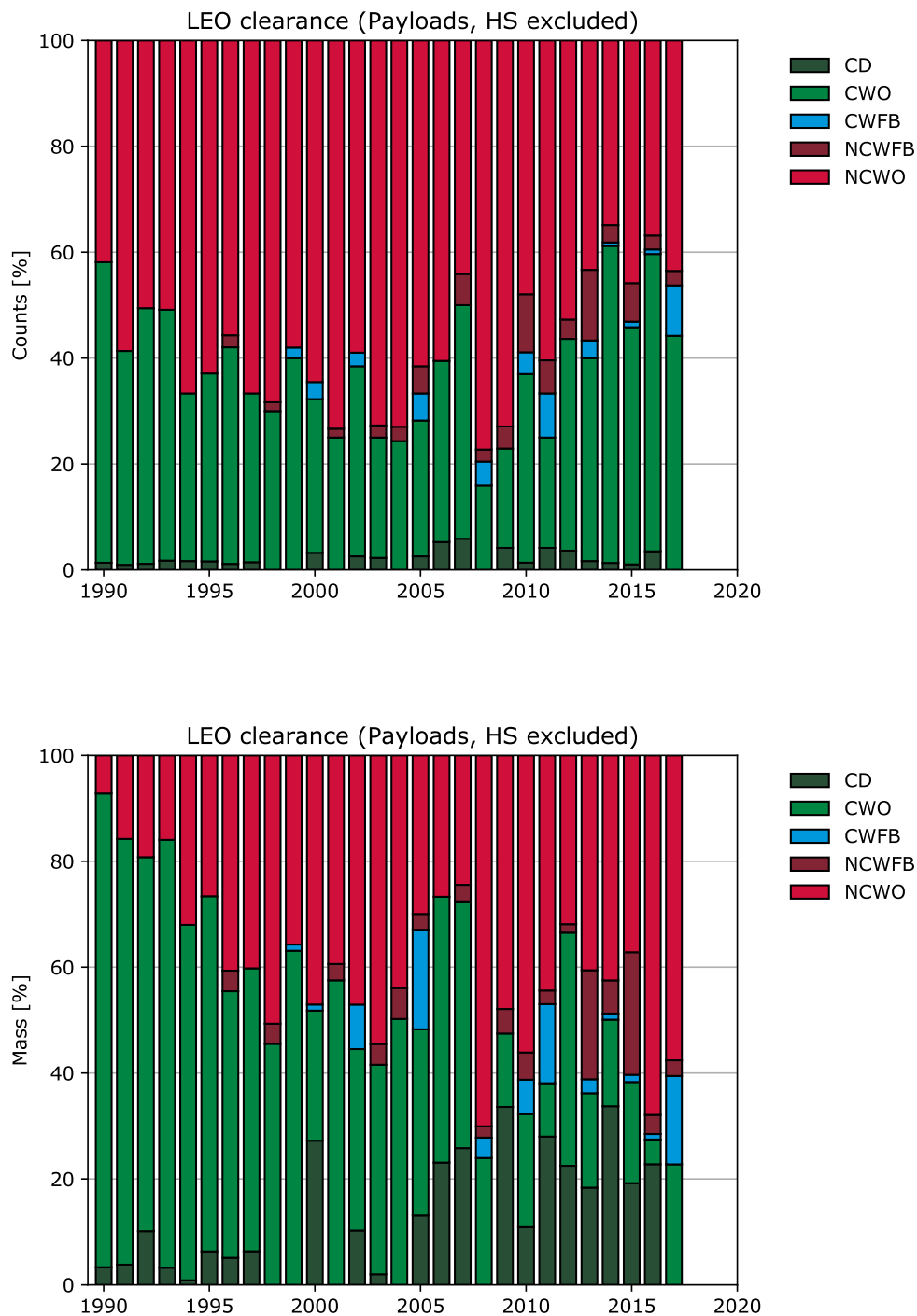
Figure 6.2: Relative share in terms of number (top) and mass (bottom) of disposal behaviour classes for payloads in LEO, excluding objects associated with human spaceflight.
