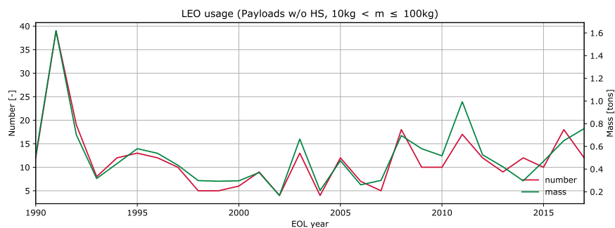
(b) Between 10.0 and 100.0 kg
