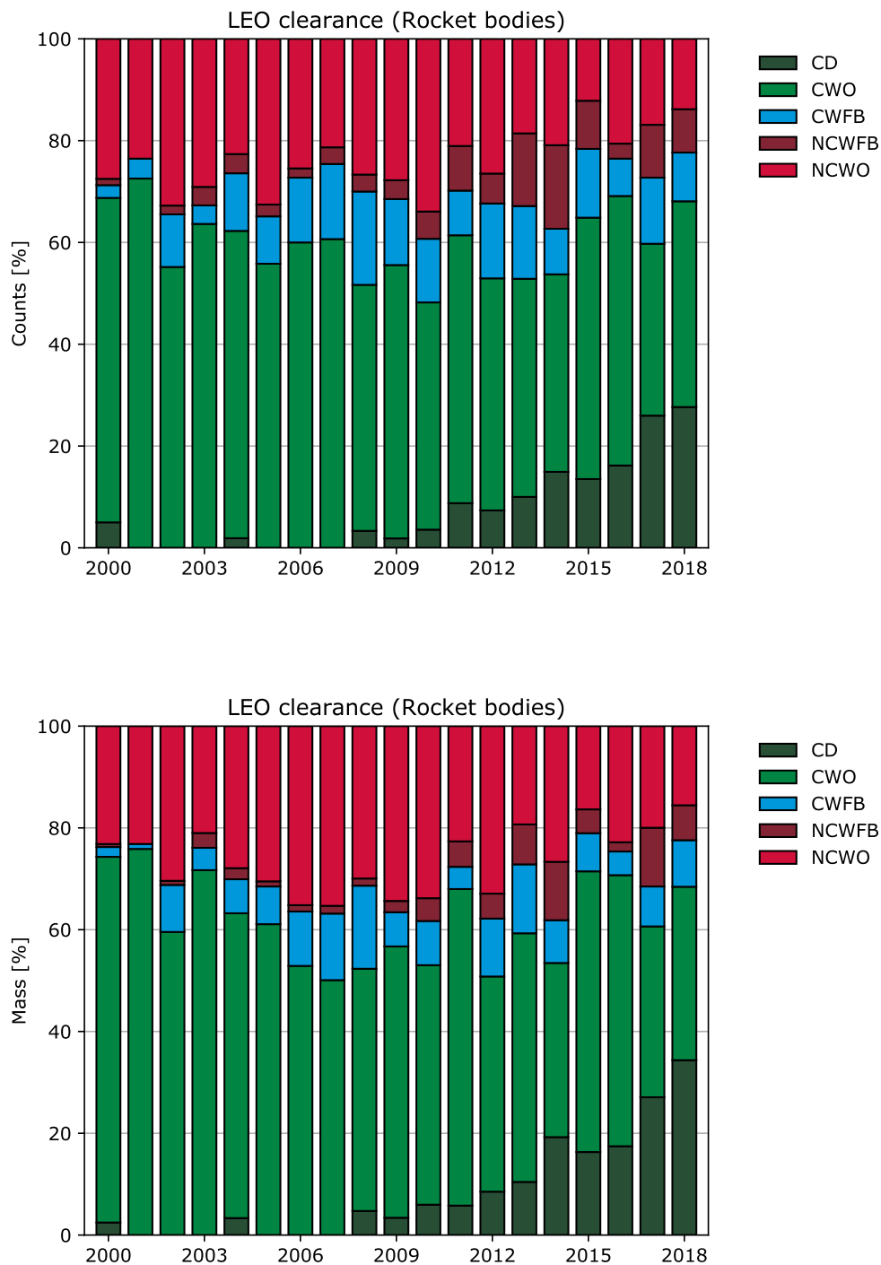
Figure 6.3: Relative share in terms of number (top) and mass (bottom) of disposal behaviour classes for Rocket Bodies in LEO.
