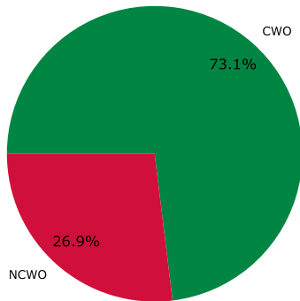
LEO compliances (Payloads w/o HS, EOL \geq 1990, m \leq 10kg)
