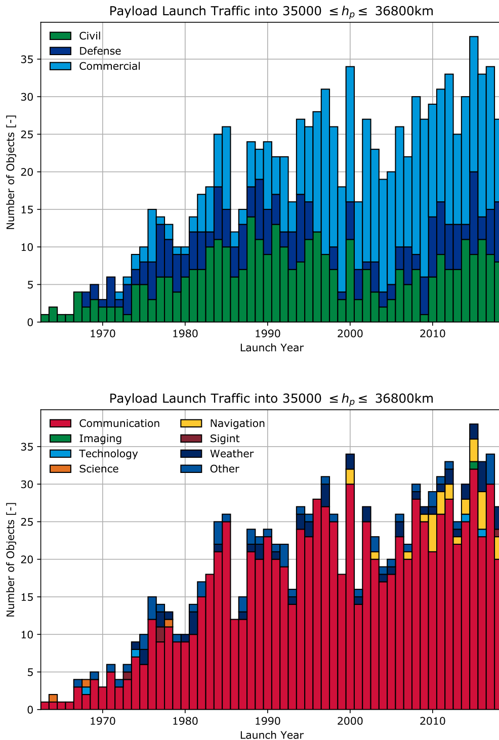
Figure 2.10: Evolution of the launch traffic near \text{GEO}_{\text{IADC}} per mission funding (top) and type (bottom).
