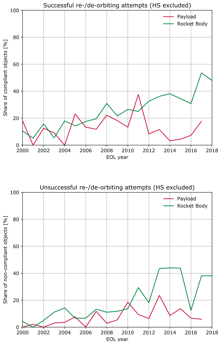
Figure 6.4: Relative shares of success w.r.t. compliance (top) and non-compliance (bottom), excluding objects associated with human spaceflight.
