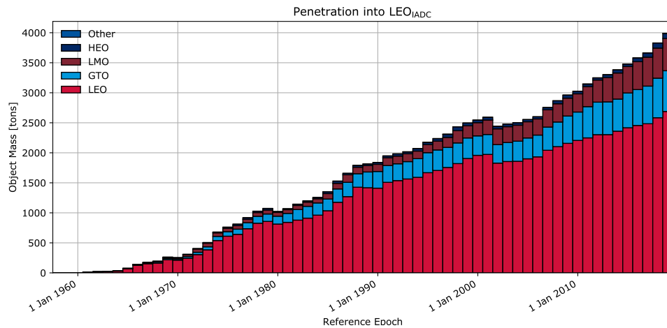
(b) Evolution of absolute mass.
