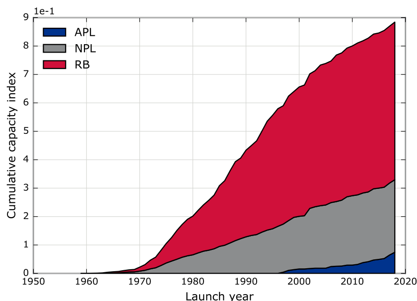
Figure 7.1: Distribution of the capacity use among rocket bodies (RB), inactive payloads (NPL) and active payloads (APL).
