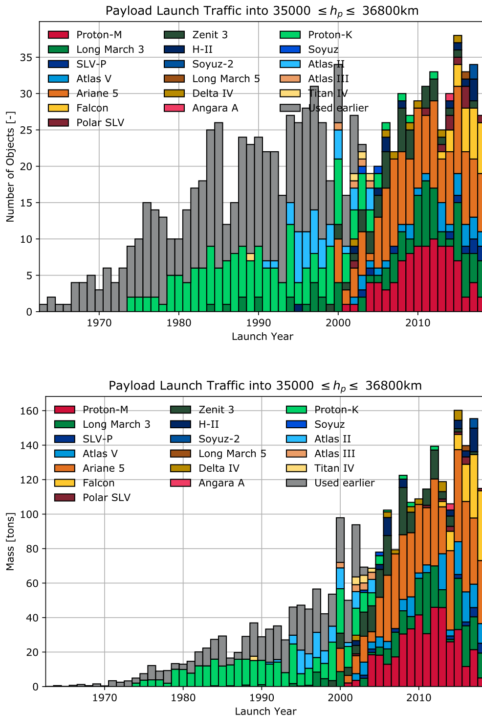
Figure 2.11: Evolution of the launch traffic near \text{GEO}_{\text{IADC}} per launcher family expressed in terms of number of objects (top) and mass (bottom).
